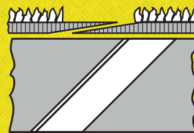
Type 5 Overlapping glued joint. Grit zone is completely ground off. Preferred joint for wood finishes with flat contact elements
